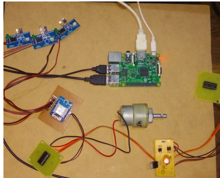
Fig2:- hardware of proposed system
